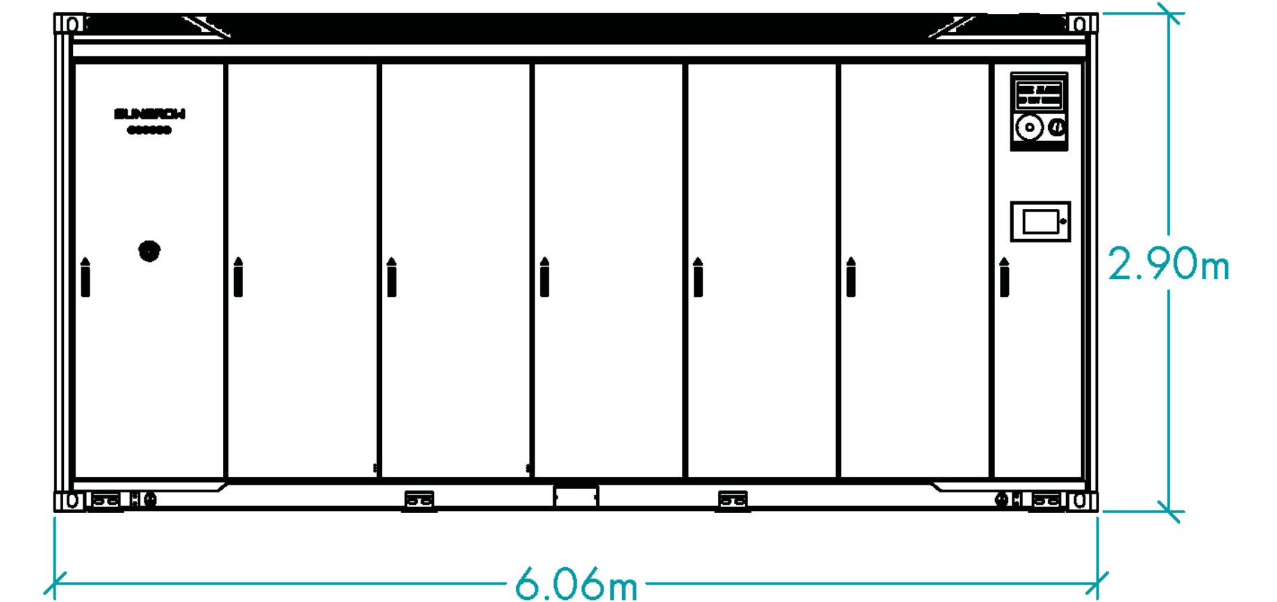
Front View
